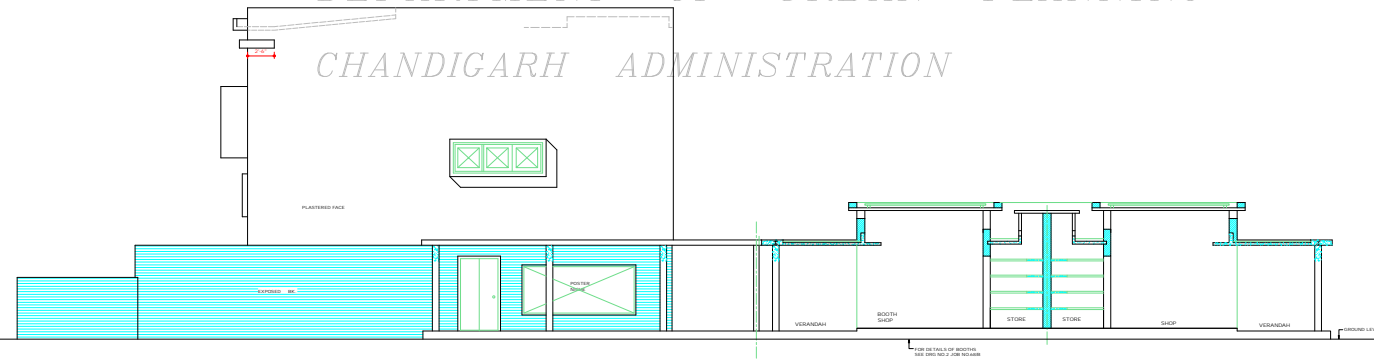
SECTIONAL ELEVATION AT JUNCTION (A)
