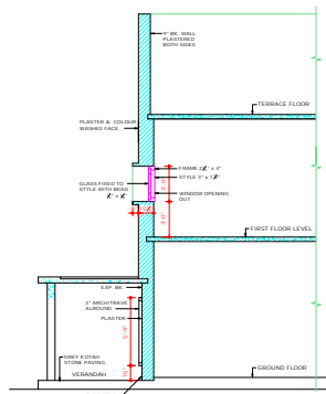
SECTION AT B-B'
