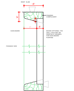
DETAILED SECTION OF SIGN BOARD
