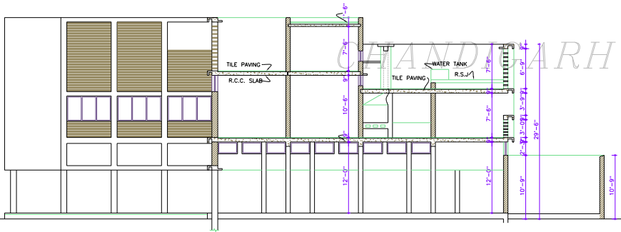
SECTIONAL ELEVATION A-B
