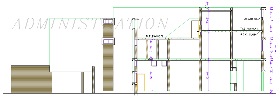
SECTIONAL ELEVATION C-D
