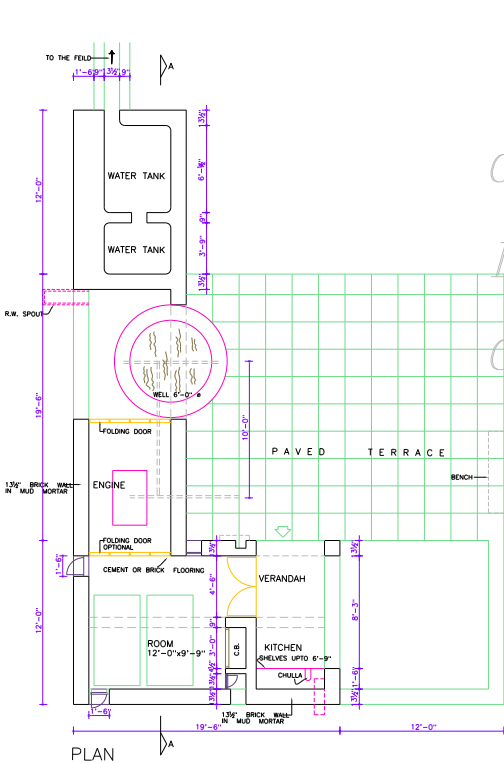
PLAN
